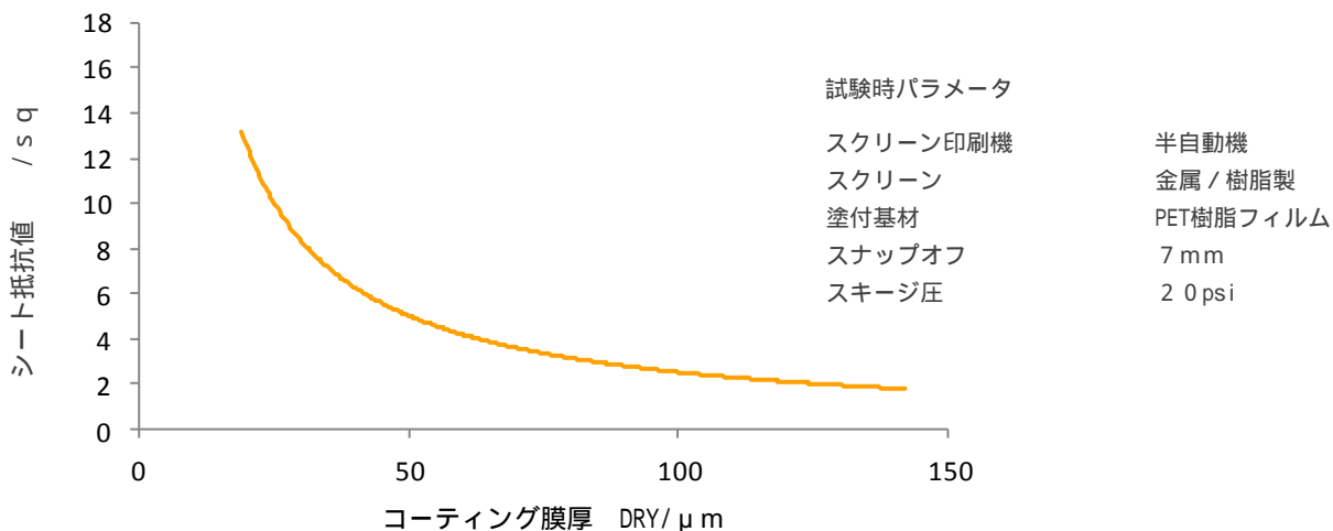
Fig. 1: Dependency of sheet resistance vs. coating thickness
